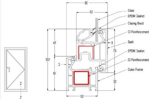
NOTE: All measurements are in MM Cross Section of Outside Openable Window
