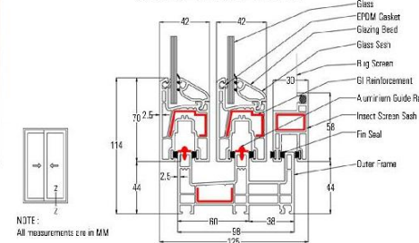
Sliding Window
